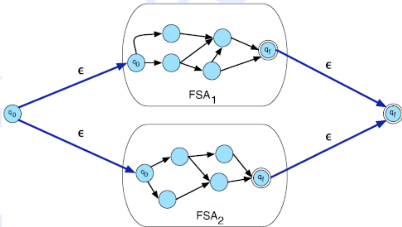
The union ( \cup ) of two FSAs.
